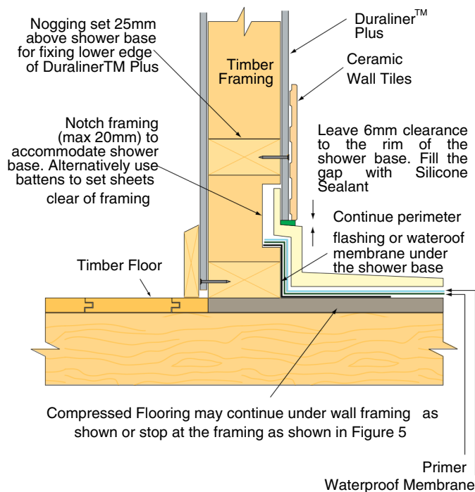
FIGURE 4 // PREFORMED SHOWER BASE
