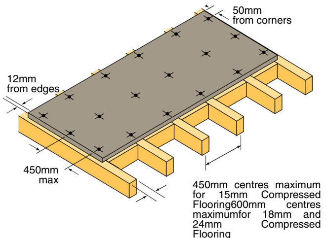
FIGURE 9 // FIXING PATTERN
