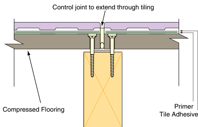
FIGURE 7 // CONTROL JOINTS
