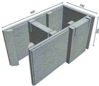
VERSALOC LEFT-HAND CORNER BLOCK
